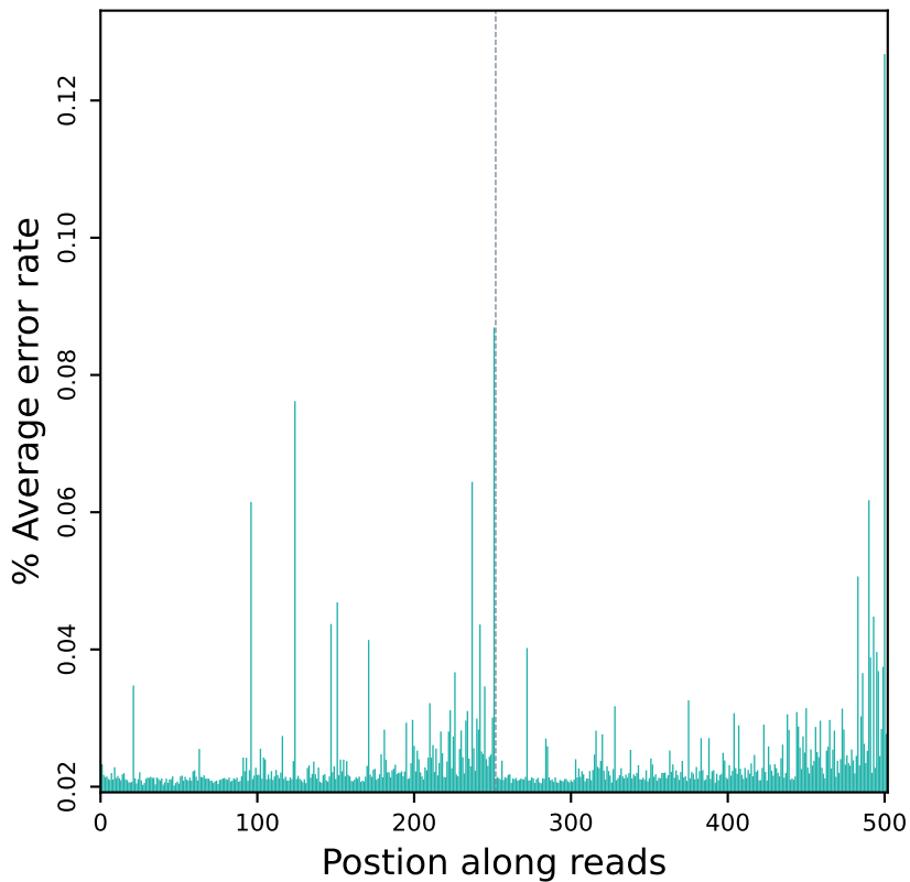
Error rate distribution along reads (R10513)
